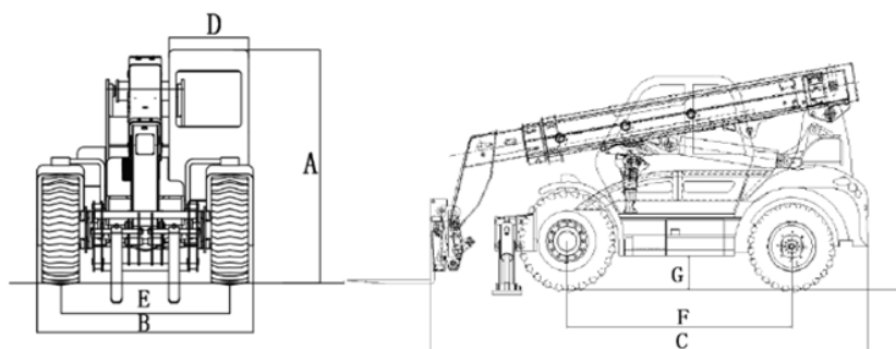
Fig. 1-1 Overall size
